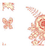
001 Mustard Gas
